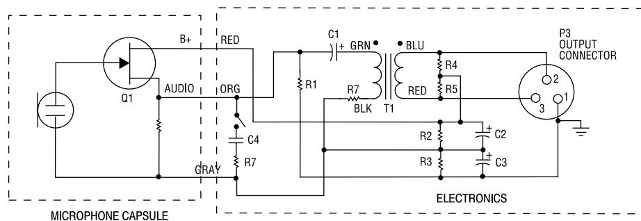
PZM-30D Schematic
