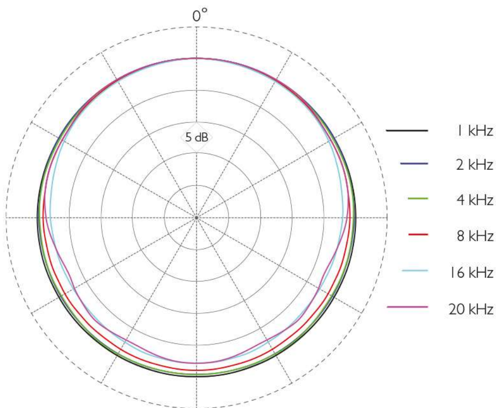
Typical response of a 4060
