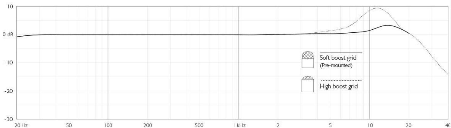
Typical response of a 4060
